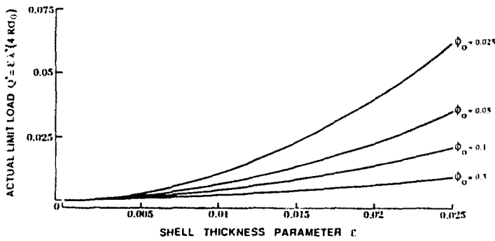
Fig. 5(b). Actual limit load as a function of the non-dimensional shell thickness for representative values of the angular size of the cut-out. The curves are generated by using the numerical solution for \lambda^* (shown in Fig. 5(a)) in eqn (33). The constant multiplier 4R\sigma_0 is taken to be unity.
